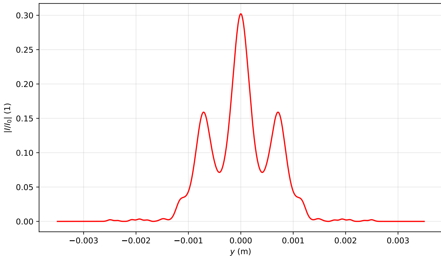
Intensity profile I(x=0, y, z=1.911)/I_0 , P_{in}=7.0P_{cr} , artificial time
